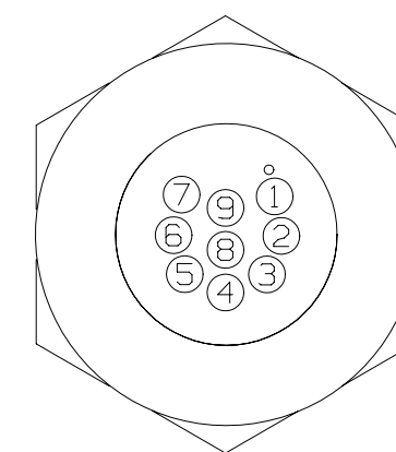
9F-A CONNECTOR PANEL MOUNT
