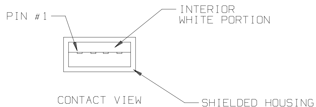
4 PIN PLUG USB "A" CONNECTOR
