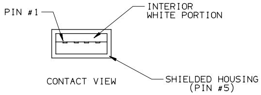
4 PIN PLUG USB "A" CONNECTOR
