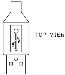
4 PIN PLUG USB "A" CONNECTOR
